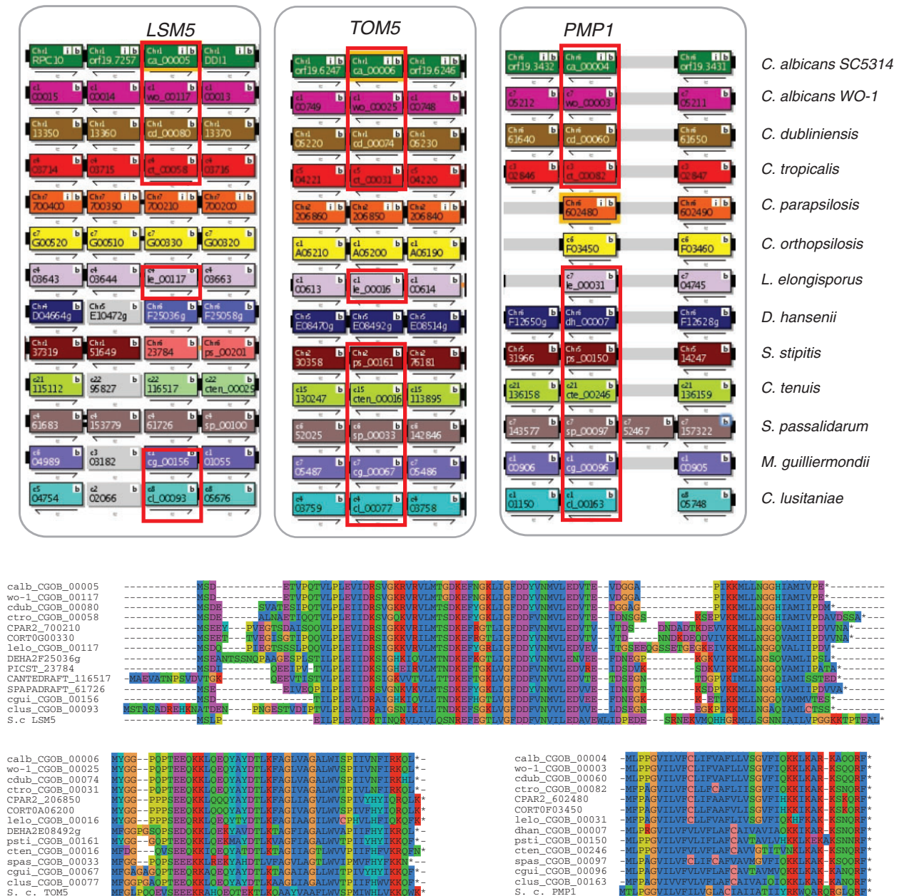
Fig. 2. Gene finding in Candida species. Examples of three small genes (orthologs of LSM5, TOM5, and PMP1 from Saccharomyces cerevisiae ) identified in multiple Candida species. The upper panels show screen shots from CGOB. The genes highlighted in red were identified by SearchDOGS. The lower panels show multiple alignments of the predicted protein sequences carried out using SeaView (Gouy et al. 2010). The species are listed in the same order as in the top panels (S.c. = Saccharomyces cerevisiae ).
